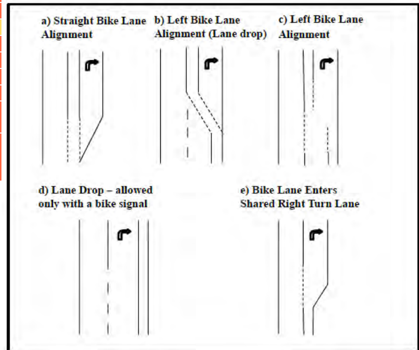
Figure 2 Right Turn Lane Configuration Types 2
